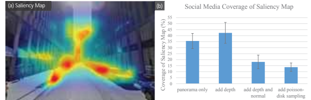
Figure 7: (a) Street view with saliency map overlay. The visualization has a red-yellow-green-transparent scheme, where red indicates high saliency and transparent indicates low-saliency. (b) Evaluation results of saliency coverage from 100 immersive GSV panoramas.
